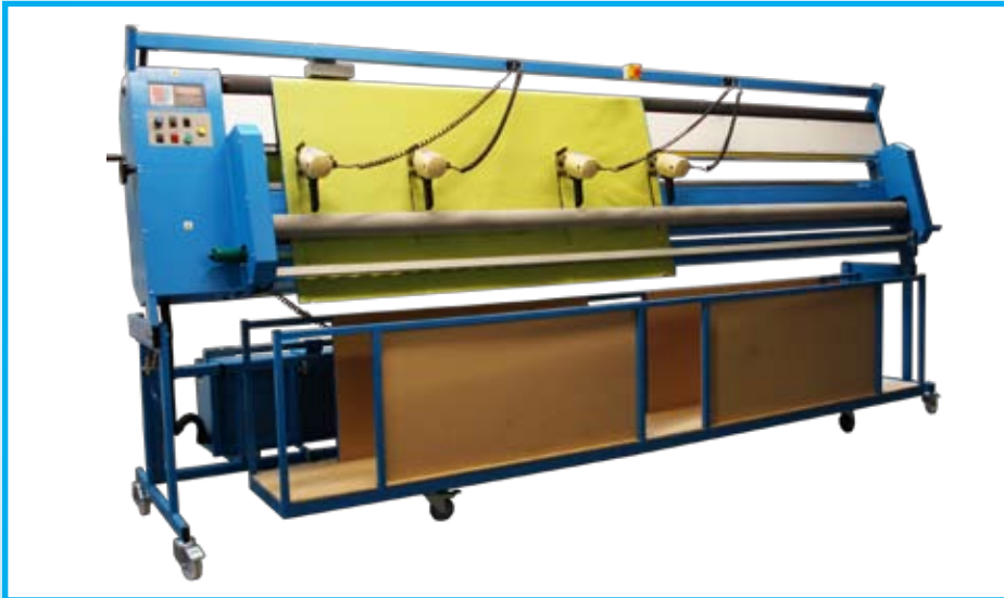
AM featuring additional vertical cutters, edge guidance, power cutter, and collection trolley
